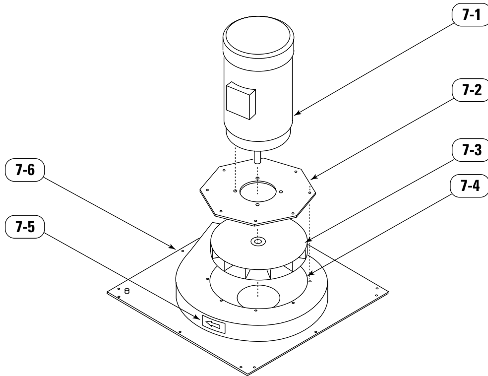
Parts Drawing 7, Power Pack Assembly
