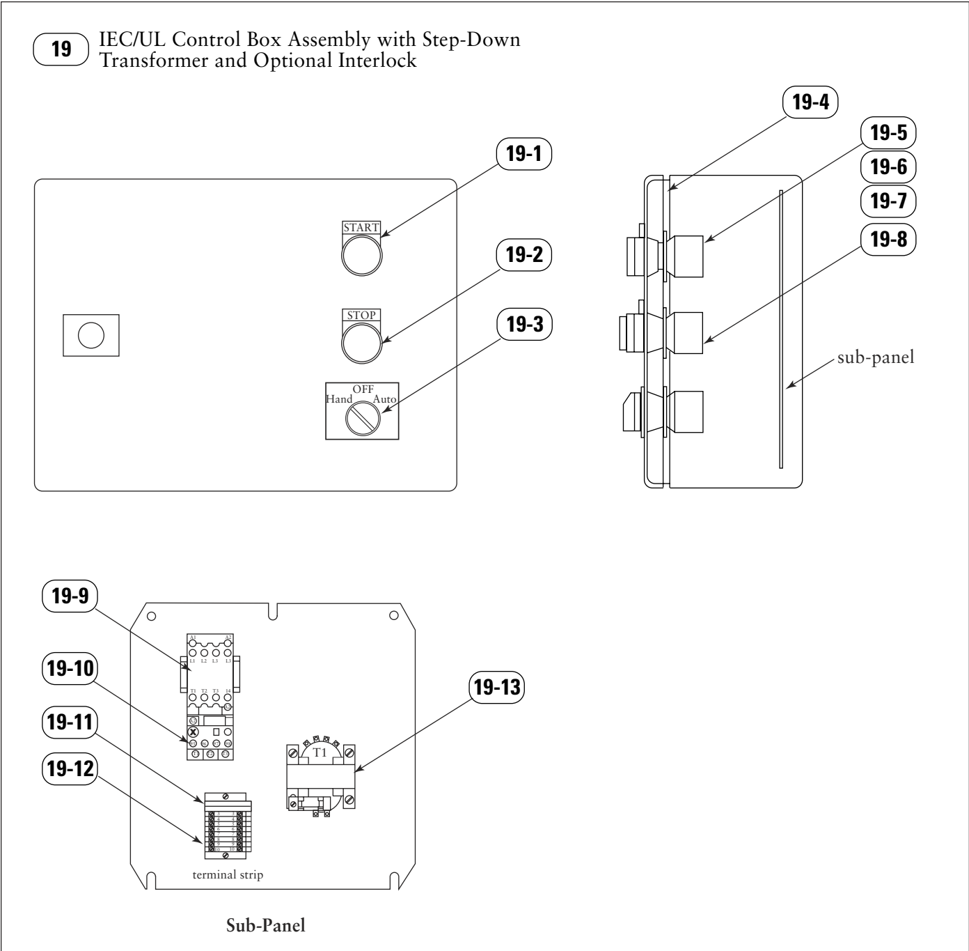
Parts Drawing 19, IEC Control Box Assembly with Step-Down Transformer and Optional Interlock
