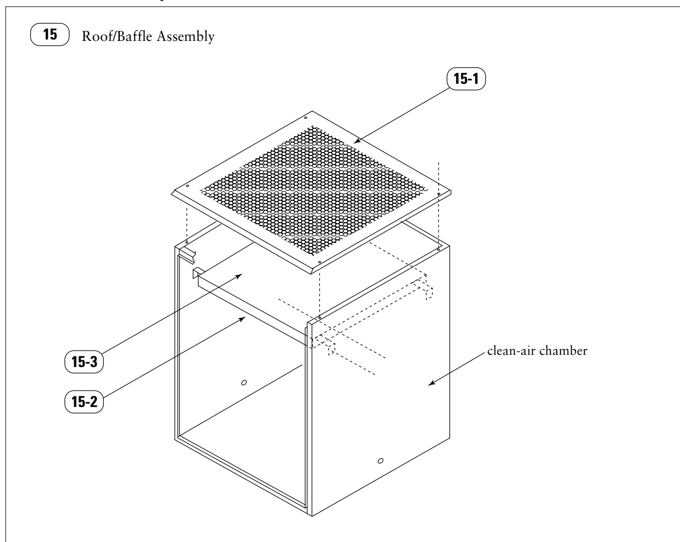
Parts Drawing 15, Roof/Baffle Assembly
