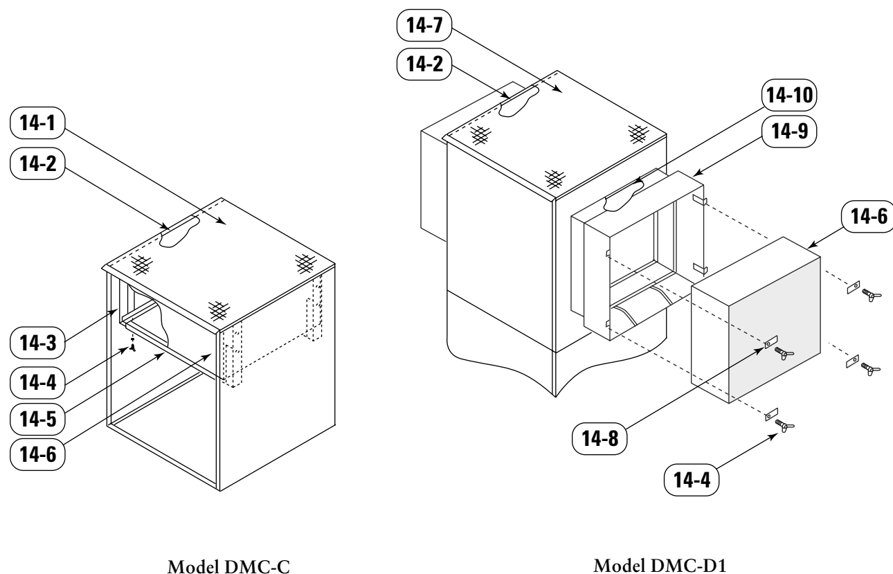
Parts Drawing 14, HEPA Filter Assembly
