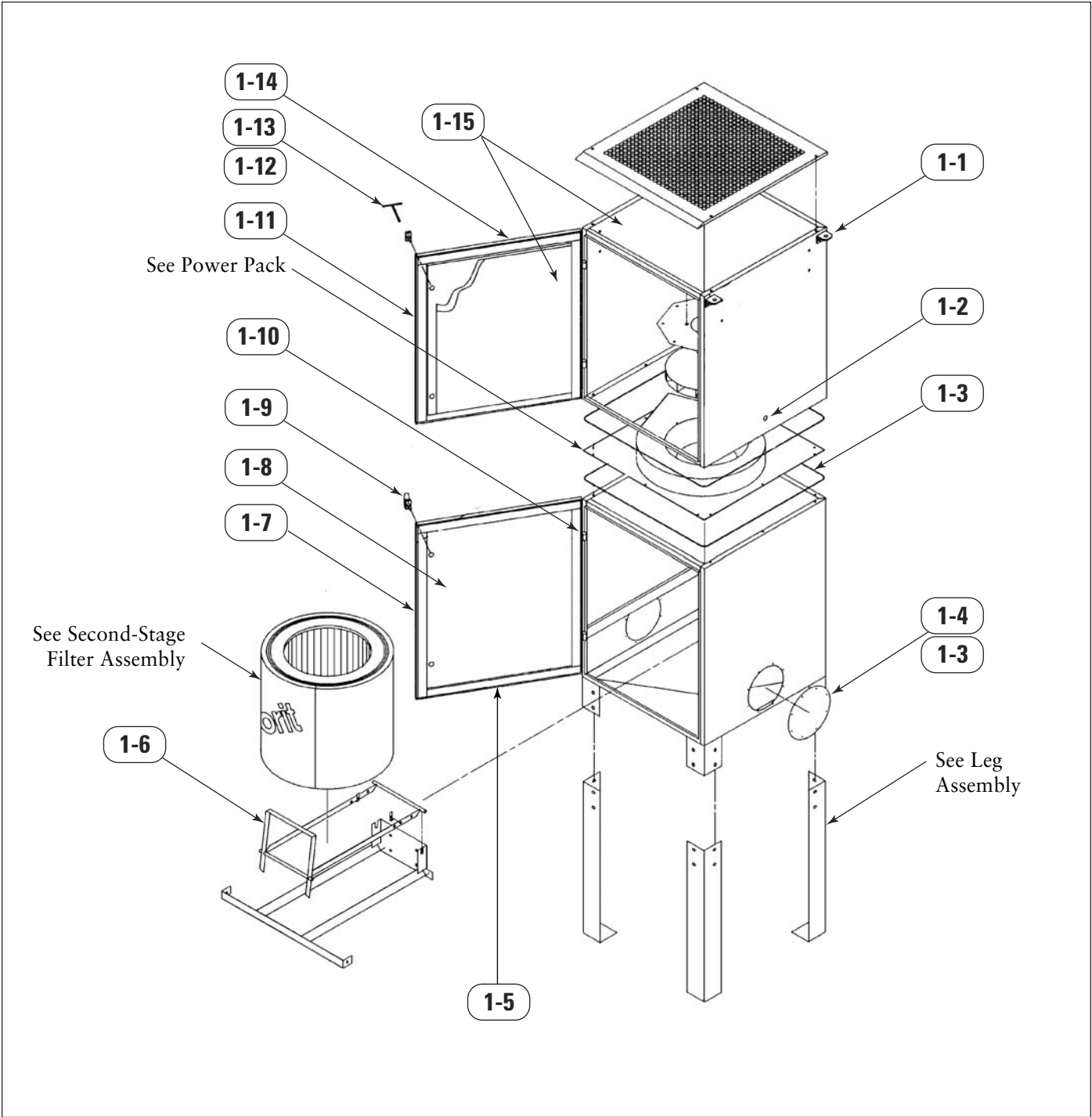
Parts Drawing 1, Dryflo Mist Collector
