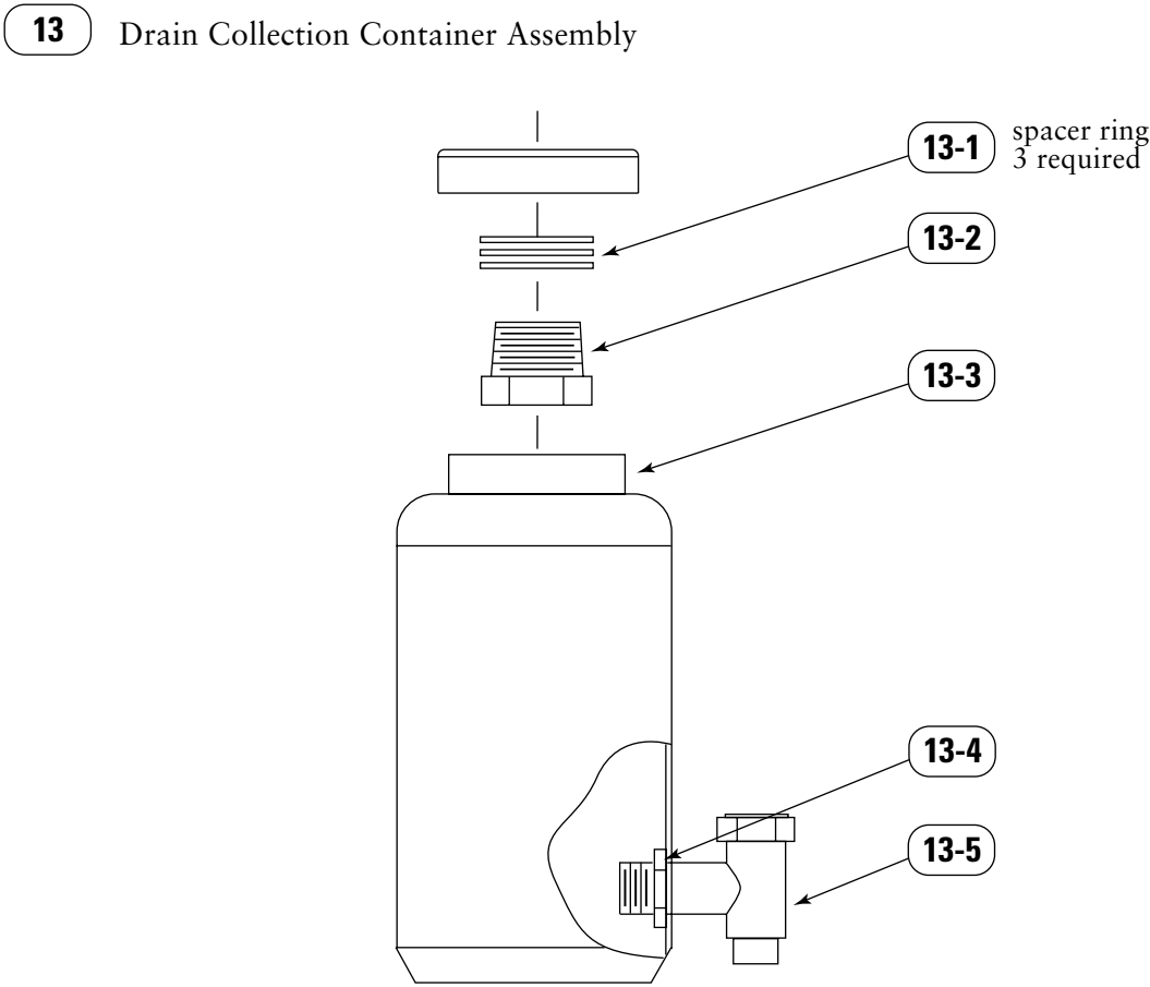
Parts Drawing 13, Drain Collection Container
