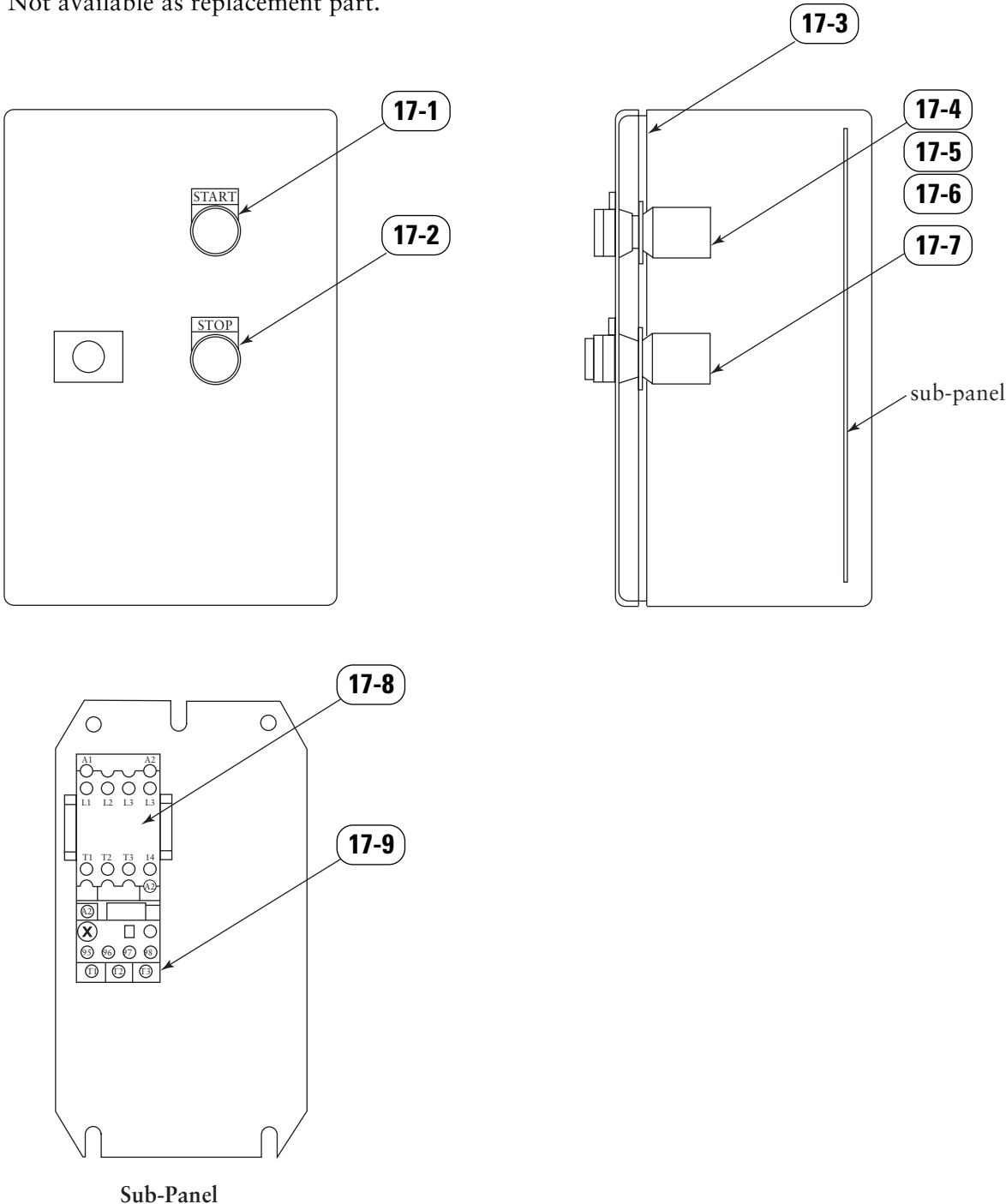
Parts Drawing 17, IEC/UL Control Box
