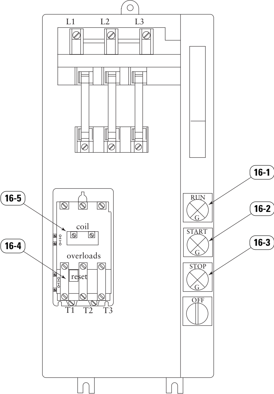
Parts Drawing 16, NEMA Control Box
