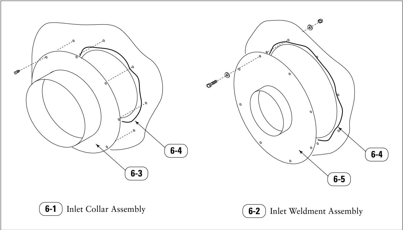
Parts Drawing 6, Inlet Assembly
