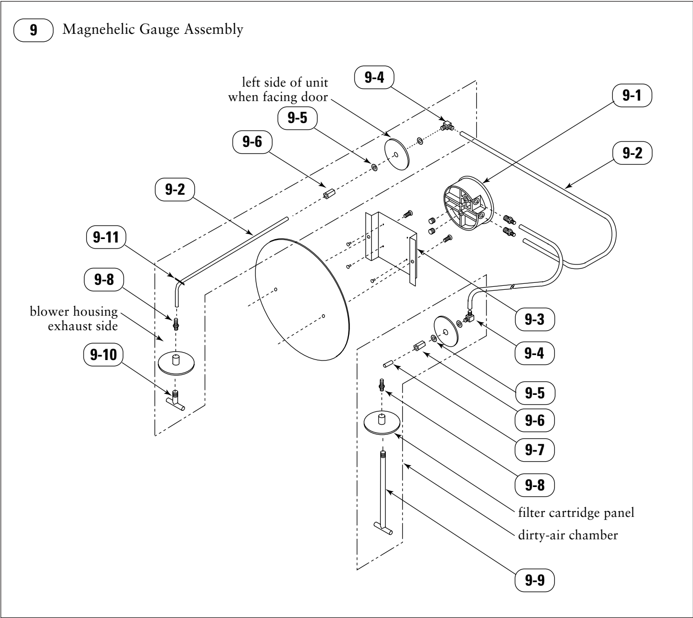
Parts Drawing 9, Remote-Mount Magnehelic Gauge
