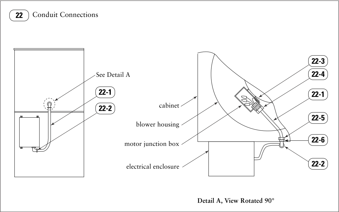
Parts Drawing 22, Conduit Connections
