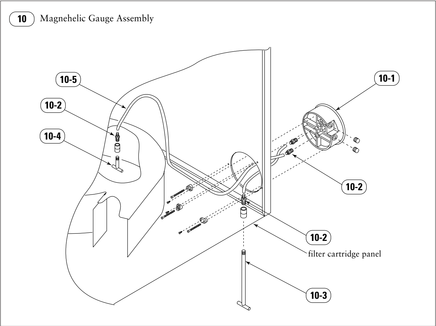
Parts Drawing 10, Door-Mount Magnehelic Gauge
