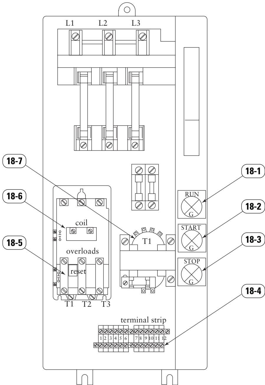
18 NEMA Control Box Assembly with Step-Down Transformer and Optional Interlock
