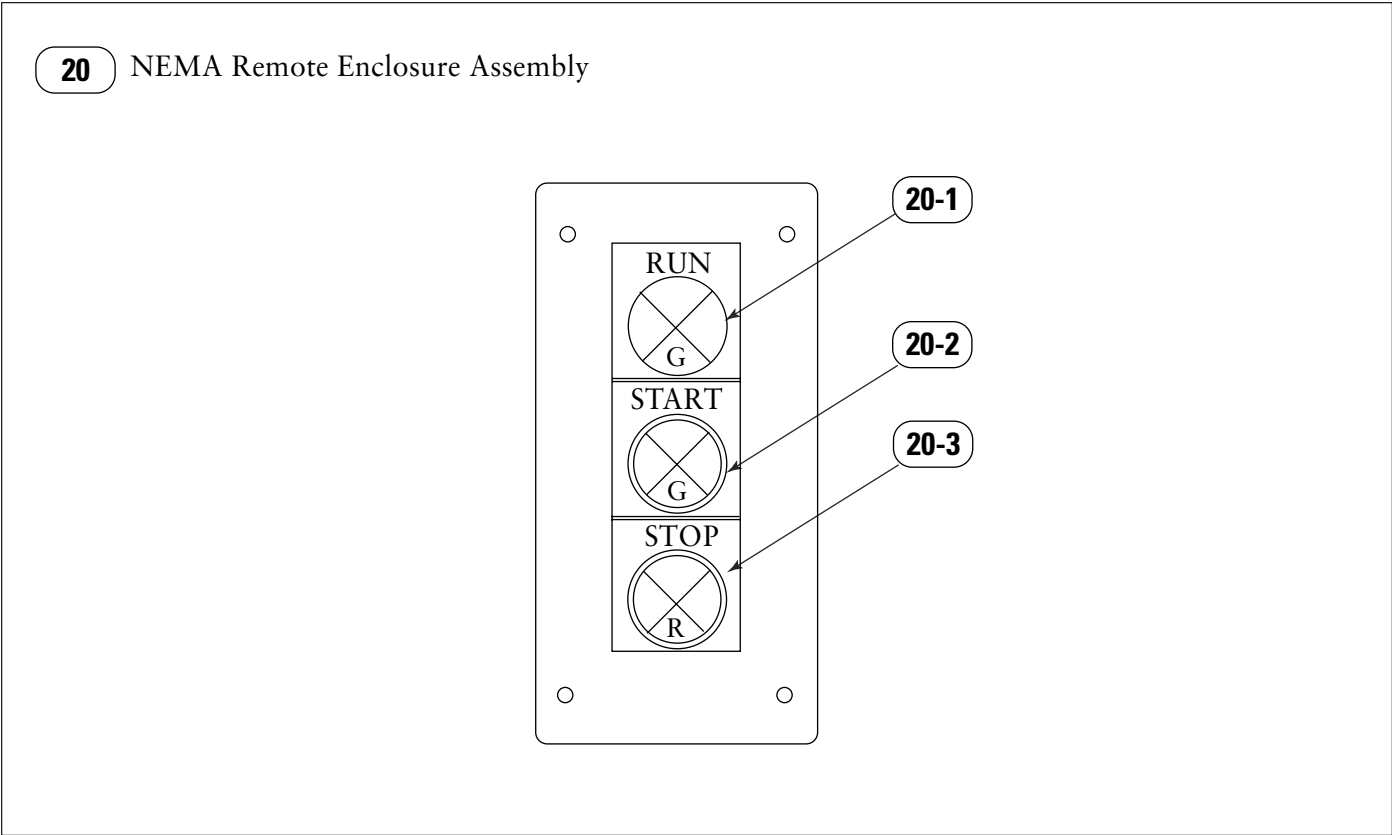
Parts Drawing 20, NEMA Remote Enclosure Assembly
