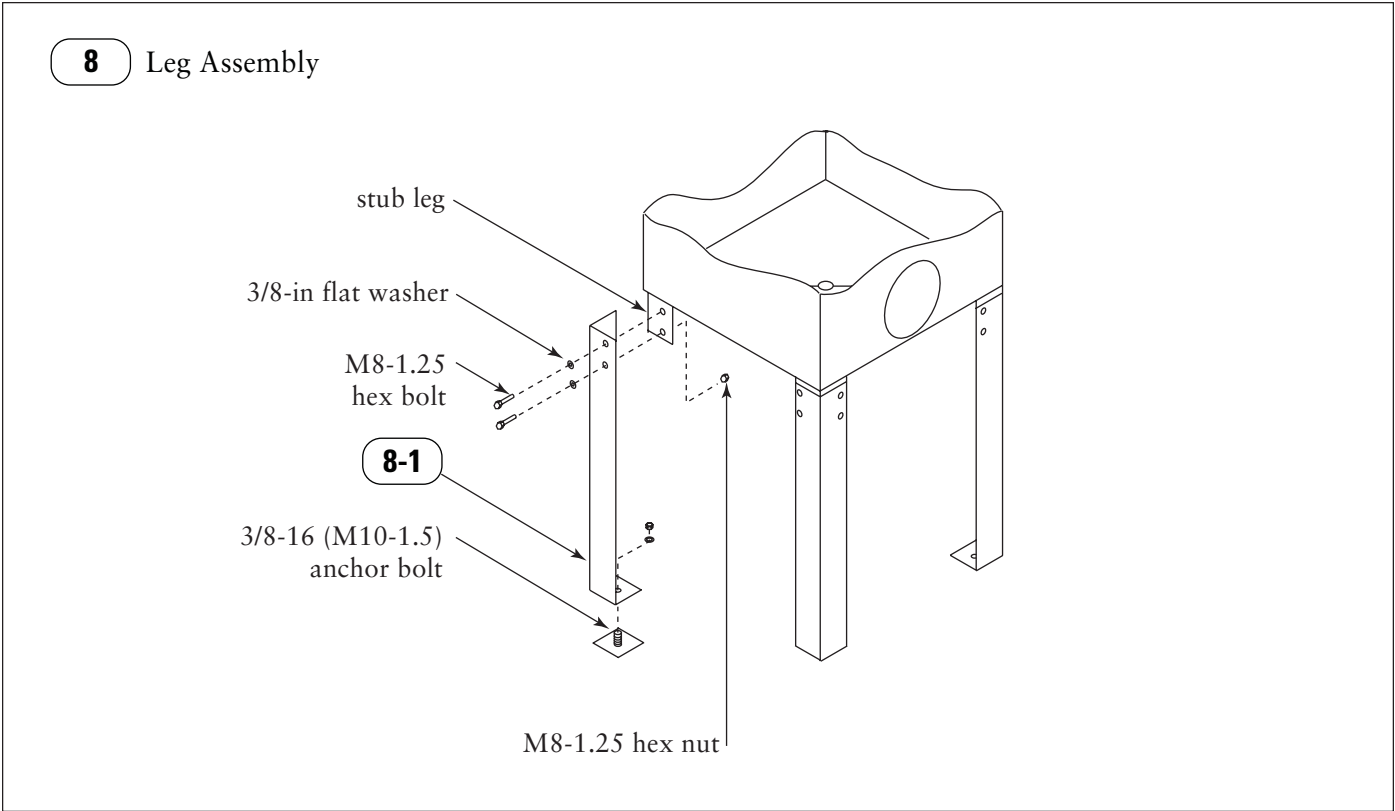
Parts Drawing 8, Leg Assembly
