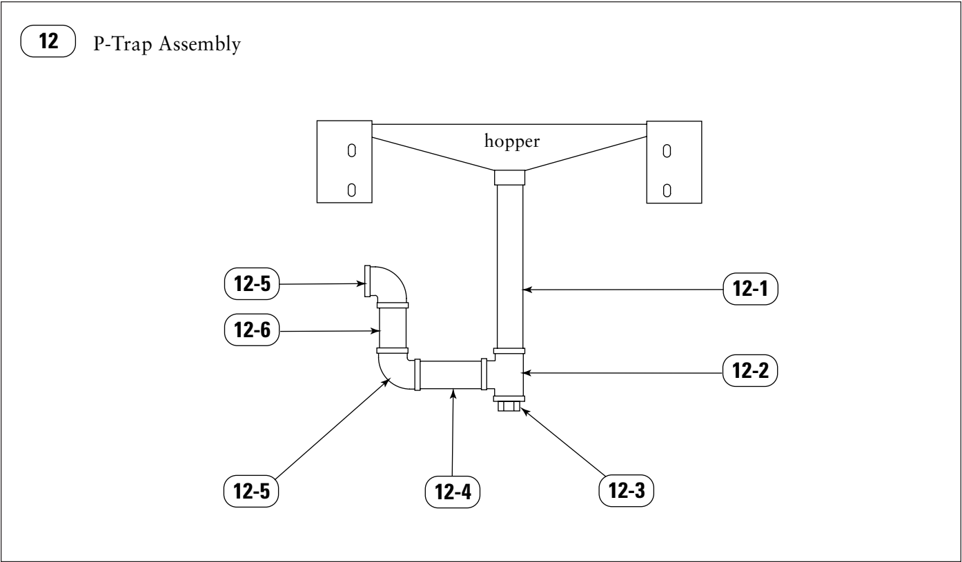
Parts Drawing 12, P-Trap Assembly
