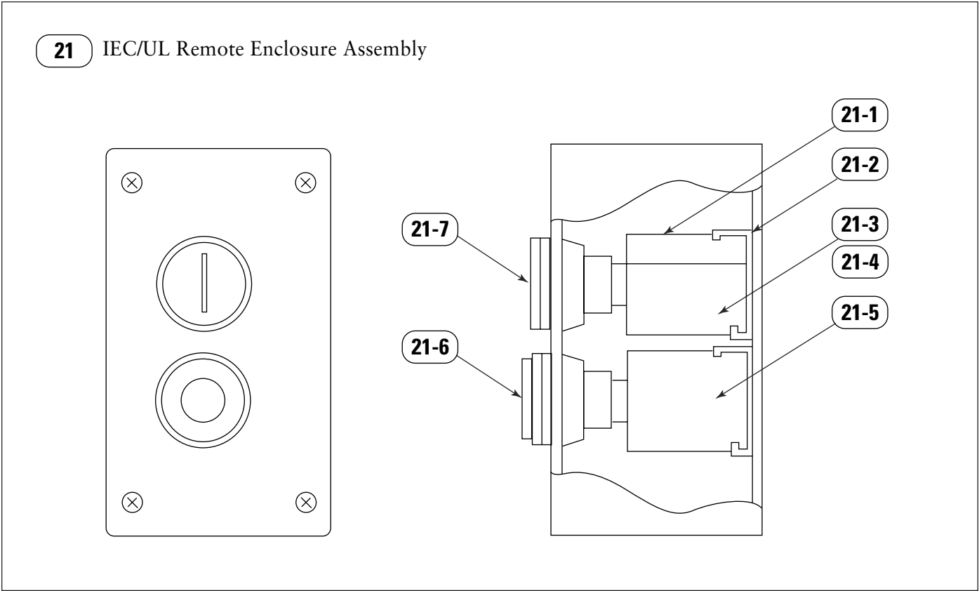
Parts Drawing 21, IEC/UL Remote Enclosure Assembly
